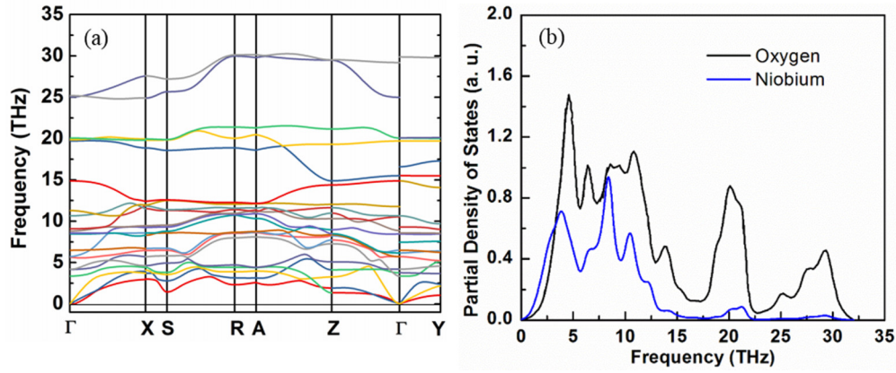
FIG. 2. DFT calculated (a) phonon dispersion relation and (b) partial phonon density of states of \text{Nb}_2\text{O}_5 .
