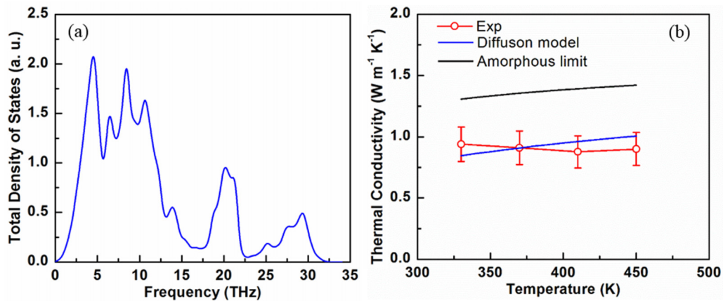
FIG. 6. (a) Total vibrational DOS from DFT calculation. (b) Temperature-dependent thermal conductivity. Two minimum thermal conductivity models are calculated to compare with the experimental values.
