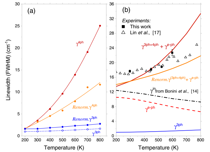
FIG. 2. (a) Intrinsic E_{2g} mode linewidth from ph-ph interactions \gamma^{\text{ph-ph}} , with and without phonon renormalization. Here, the data with “Renorm.” at the beginning of the label are those calculated with TDEP to account for the temperature effect, and Renorm. \gamma^{4\text{ph}} is fitted to a quadratic function. (b) Intrinsic E_{2g} mode linewidth of graphene from e -ph and ph-ph contributions. \gamma^{e\text{-ph}} is calculated for pristine graphene. Experiments are from Ref. [17] and our own measurements. A previous prediction [14] is plotted as the dash-dotted black line, and shows an opposite dependence on T compared to measurements.
